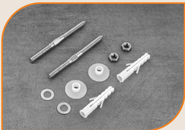
RM110 3/8 WASH BASIN BOLT(S.S) MRP:110 SIZE: 9 X 115mm
